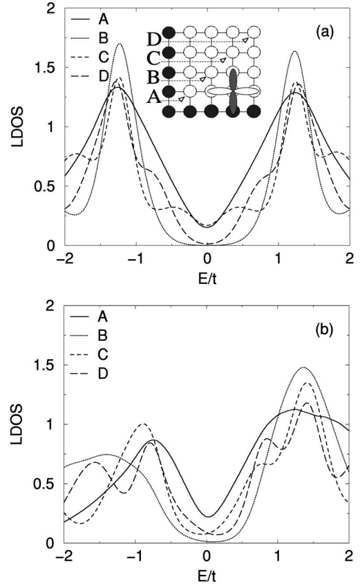
FIG. 3. The local density of states at sites A, B, C, D along the diagonal of the two-dimensional square lattice shown in the inset. (a) \mu=0 , (b) \mu=t . The chemical potential is set to \mu^I=100t at the shaded surface sites.
