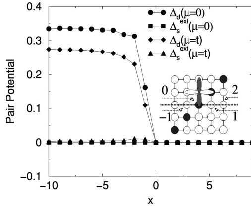
FIG. 9. The magnitude of the \Delta_d and \Delta_s^{\text{ext}} as a function of x , for the d - i - n interface shown in the inset, for \mu=0,t . The spatial distribution of impurities is indicated by solid circles, and also the labeling of the sites along the x directions is shown. The order parameter is calculated along the thick dashed line in the direction x shown in the inset.
