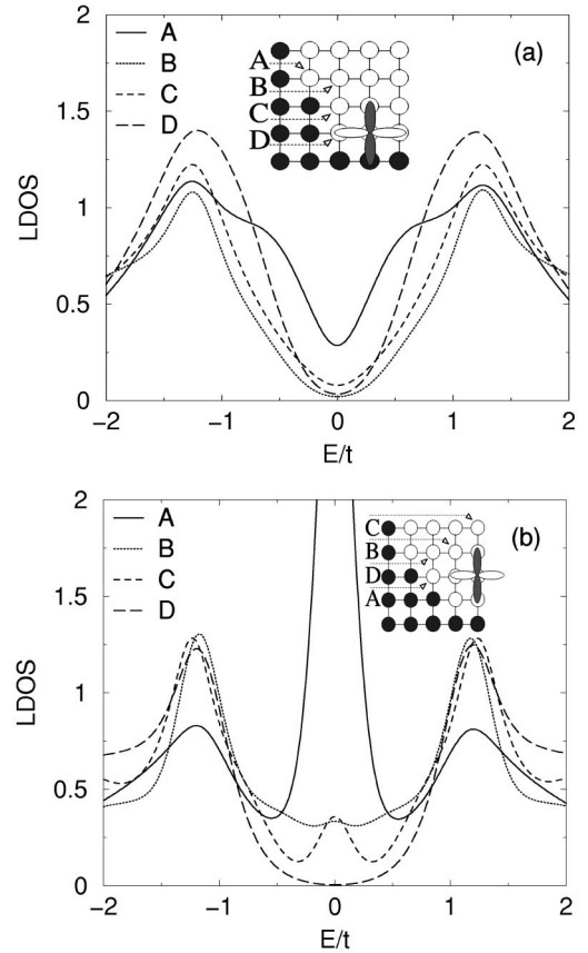
FIG. 13. (a) The local density of states at the specified sites A, B, C, D for the corner surface, with a 1 \times 2 step structure shown in the inset for \mu = 0 . The chemical potential is set to \mu^I = 100t at the shaded surface sites. (b) The local density of states at the specified sites A, B, C, D for the corner surface, with a [110] structure shown in the inset for \mu = 0 . The chemical potential is set to \mu^I = 100t at the shaded surface sites.
