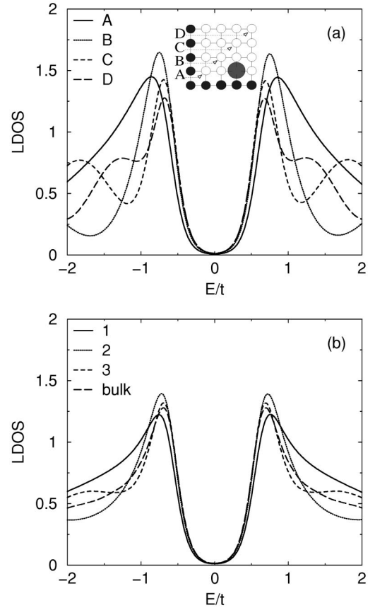
FIG. 6. (a) The local density of states at sites A, B, C, D along the diagonal of the two-dimensional square lattice shown in the inset. The pairing symmetry is s , \mu = 0 . The chemical potential is set to \mu^I = 100t at the shaded surface sites. (b) The local density of states at sites of distance x = 1, 2, 3 from the [100] surface of the two-dimensional square lattice and the bulk density of states. The pairing symmetry is s and \mu = 0 .
